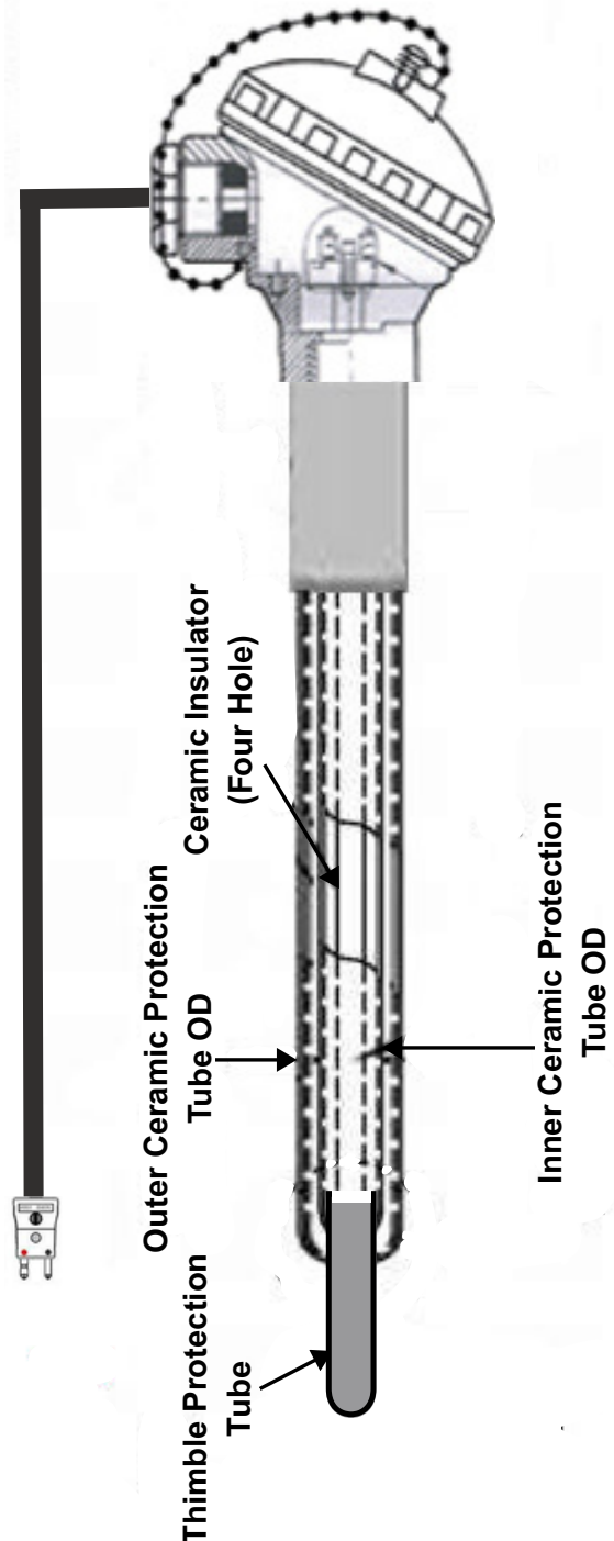
Single Level Thermocouple
