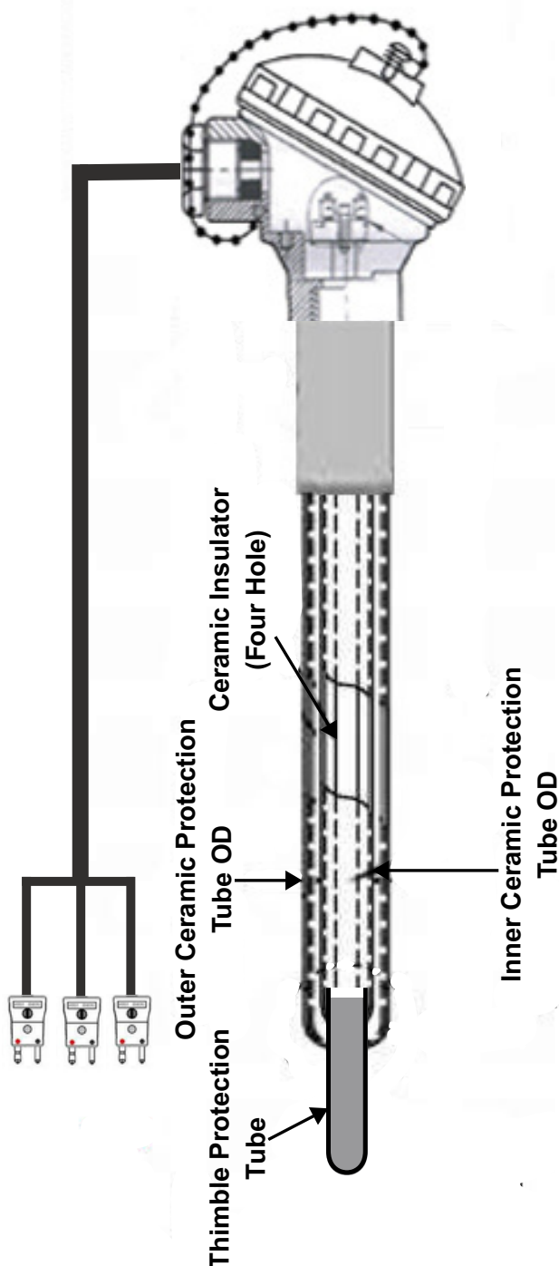
Tri Level Thermocouple
